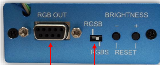
RGB OUT Sync Over Green switch
